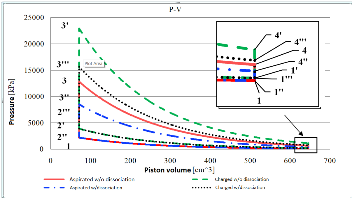
Figure 1. Theoretical p-V Otto cycles for naturally aspirated and turbocharged engines with and without dissociation
